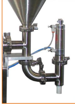
Positive cut-off filling nozzle
