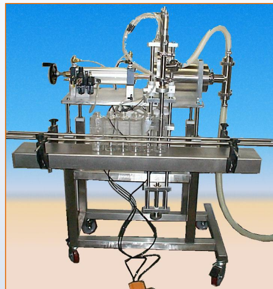
Gallon model on stand with 4 ft. ss track and diving nozzle mechanism
