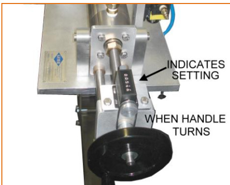
Micro fill adjustment
