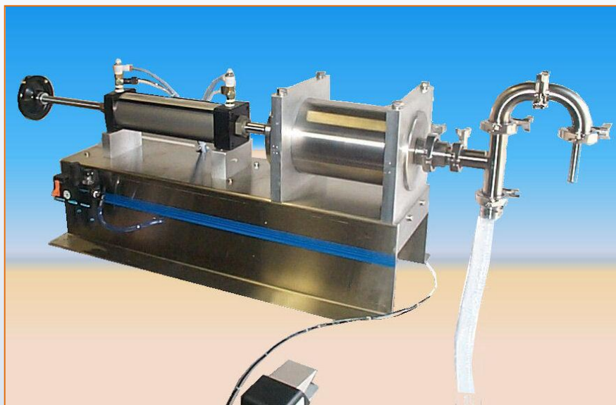
Standard table top 1 cylinder gallon filler
