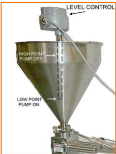
Level control
