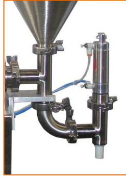
Positive cut-off filling nozzle
